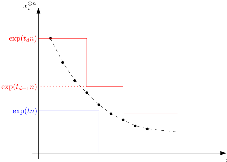
Fig. 1. Bounding the vector x^{\otimes n} by vectors with simpler profiles. The coordinates of the tensor power x^{\otimes n} are represented by dark circles, the vector used for the lower bound has only one nonzero value \exp(tn) and the upper-bounding vector has values \exp(t_d n) \geq \dots \geq \exp(t_1 n) \geq 0 .
